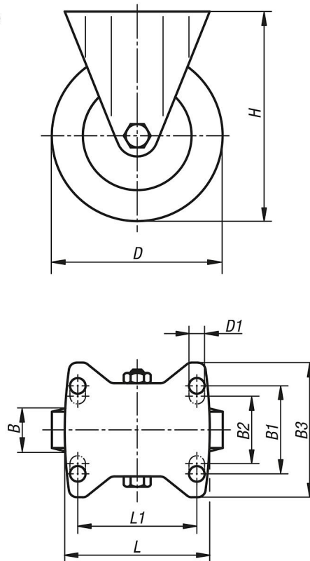
Bockrolle
