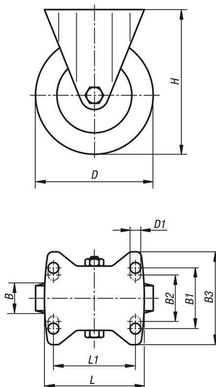
Bockrolle
