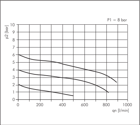
5.6. Flow characteristic
