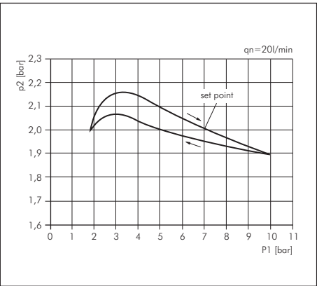
4.7. pressure characteristic
