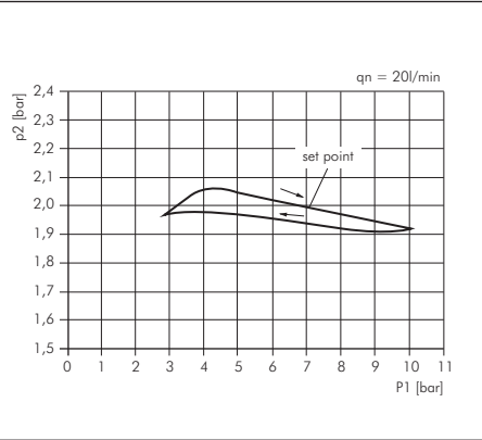
5.7. Pressure characteristic
