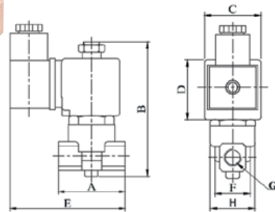
Dimensions (mm)
